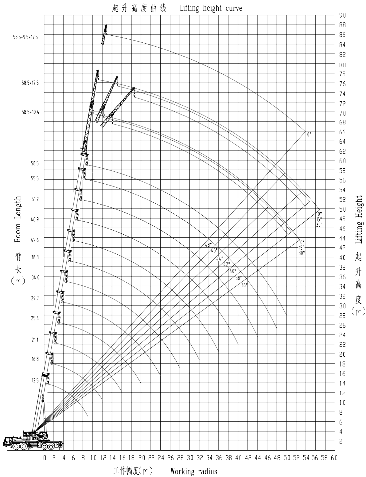
Lifting height chart with the main boom and jib installed
