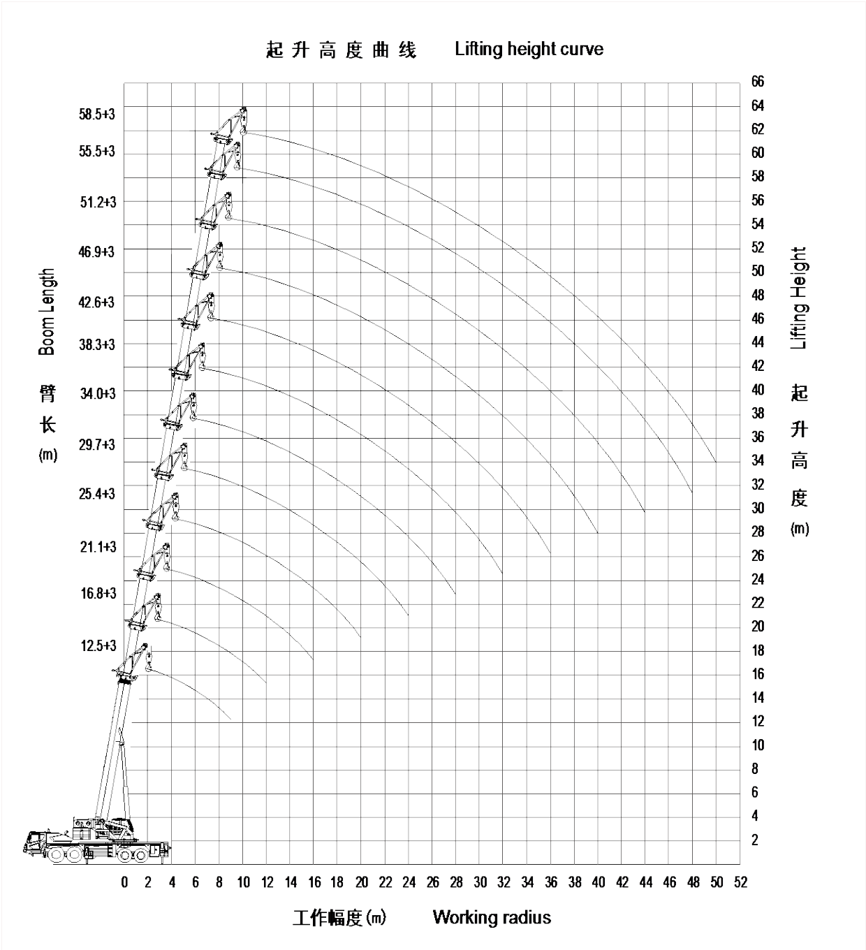
Lifting height chart with the main boom and tip boom installed
